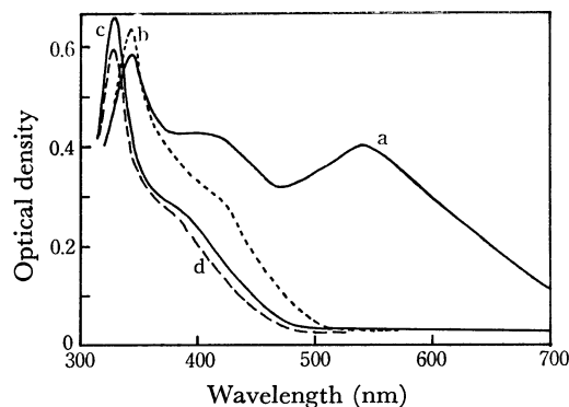
Fig. 1. Absorption spectra of \gamma -irradiated 0.08 mol% DEM in methanol at 77 K. a: sample \gamma -irradiated to a dose of 1.0 \times 10^{18} \text{ eV/g} , b: after 2 min illumination of sample a with visible light ( \lambda = 490 \text{ nm} ), c: after 2 min illumination of sample a with a visible light (no filter), d: after 60 min illumination of sample a with visible light.
